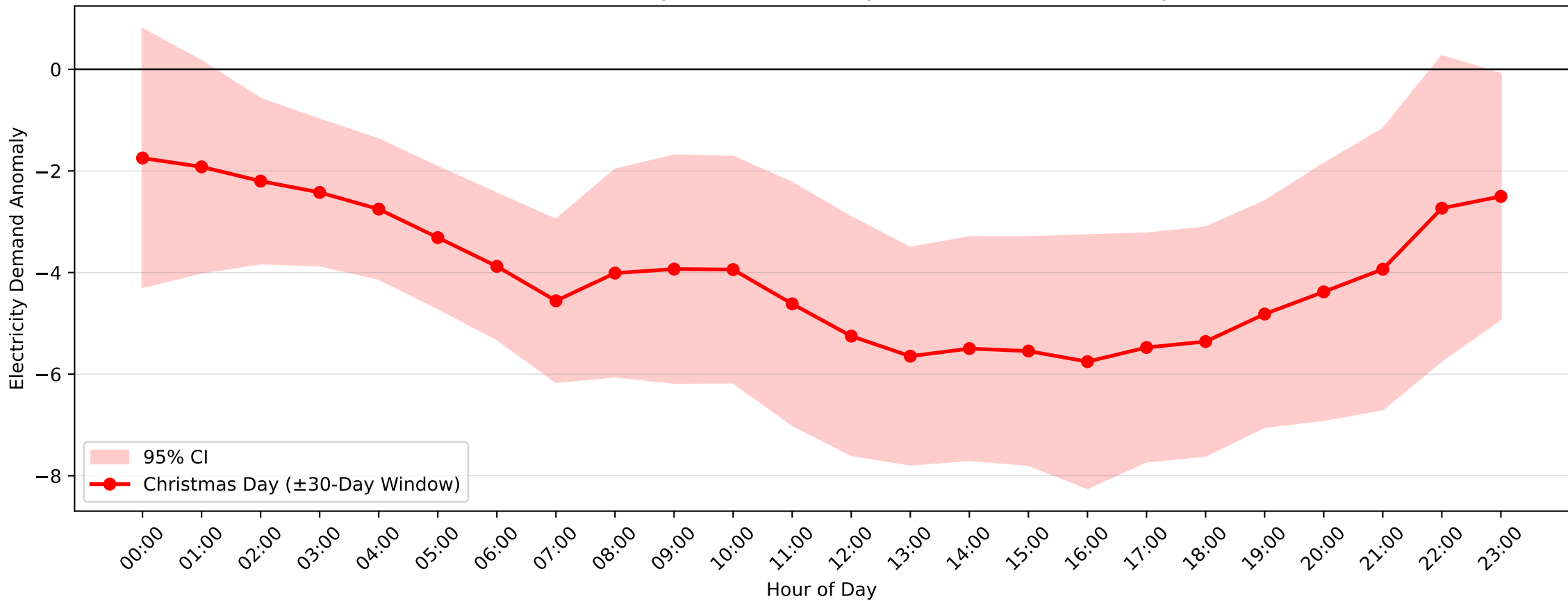
Enfield Demand Anomaly: Christmas Day (2004–2017, \pm 30 -Day Window)
